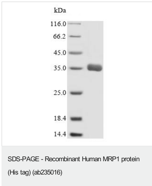
(Tris-Glycine gel) Discontinuous SDS-PAGE (reduced) analysis with 5% enrichment gel and 15% separation gel of ab235016.
