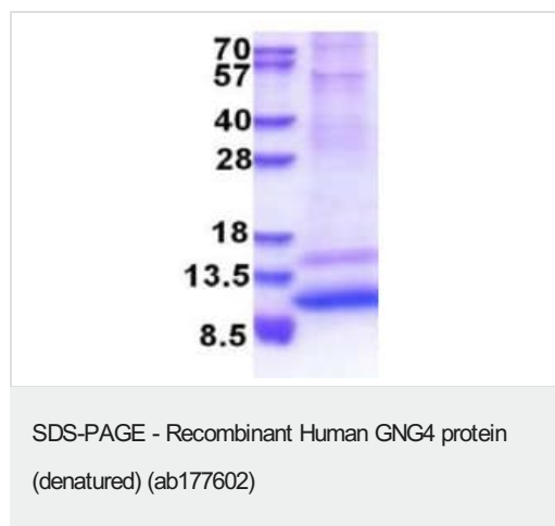
15% SDS-PAGE analysis of ab177602 (3µg).
