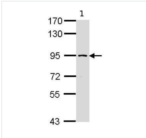
Western blot - Anti-SSRP1 antibody (ab96704)
