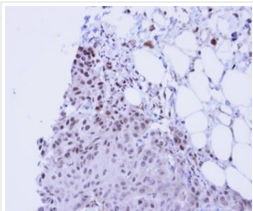
Immunohistochemistry (Formalin/PFA-fixed paraffin-embedded sections) - Anti-SSRP1 antibody (ab96704)
