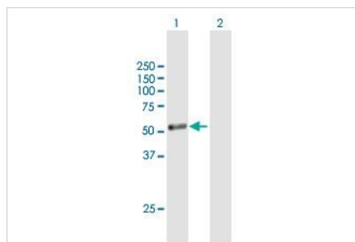
Western blot - Anti-CYP1A1 antibody (ab171883)
