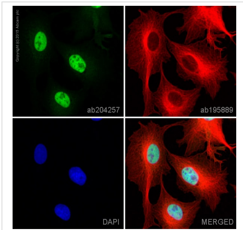
Immunocytochemistry/ Immunofluorescence - Alexa Fluor® 488 Anti-Smad3 antibody [EP568Y] (ab204257)
