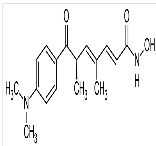
Chemical Structure - Trichostatin A (DMSO solution), histone deacetylase inhibitor (ab146598)
