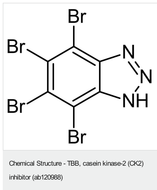
2D chemical structure image of ab120988, TBB, casein kinase-2 (CK2) inhibitor
