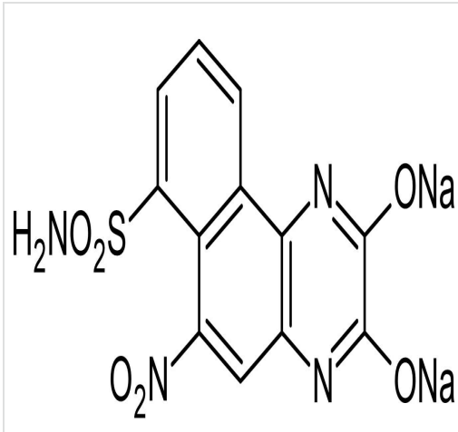
Chemical Structure - NBQX disodium salt (mM/ml), AMPA / kainate antagonist (ab144489)
