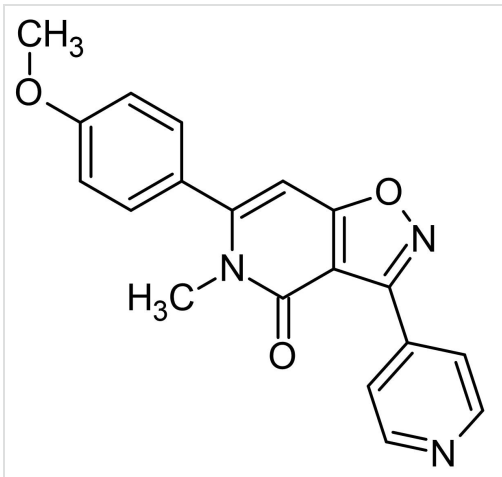
Chemical Structure - MMPIP, mGlu7 allosteric antagonist (ab120245)
