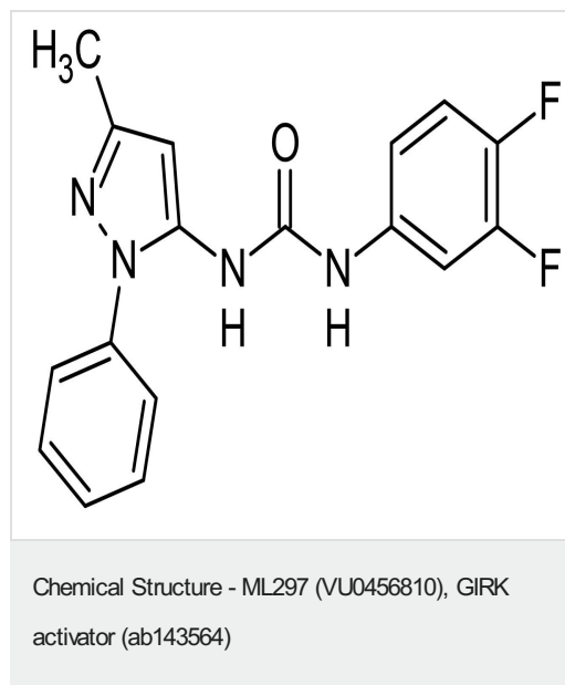
2D chemical structure image of ab143564, ML297 (VU0456810), GIRK activator
