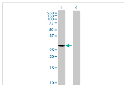
Western blot - Anti-LRRC61 antibody (ab68802)
