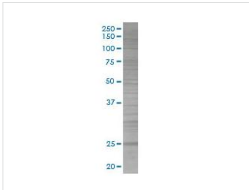
SDS-PAGE - Thymidine Kinase 1 293T Transfected Lysate - (positive control) (ab94157)
