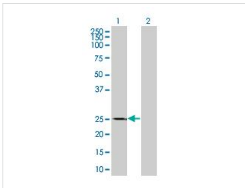
Western blot - Thymidine Kinase 1 293T Transfected Lysate - (positive control) (ab94157)
