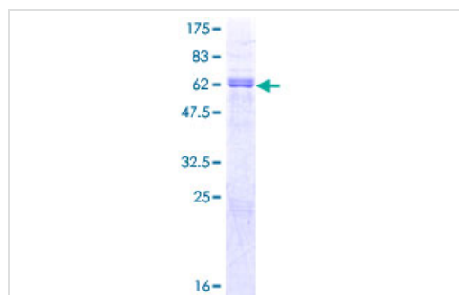
SDS-PAGE - Recombinant Human PAX9 protein (ab152592)
