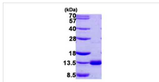
SDS-PAGE - Recombinant Human Dynein light chain protein (ab107140)
