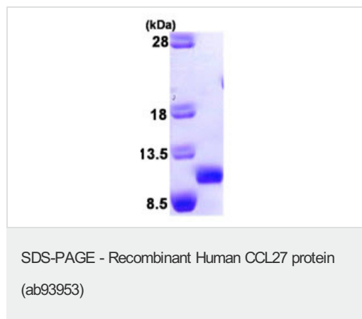
15% SDS-PAGE analysis of ab93953 (3µg)
