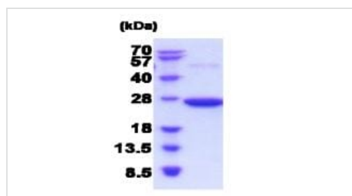
15% SDS-PAGE analysis of ab206799 (3 µg).
