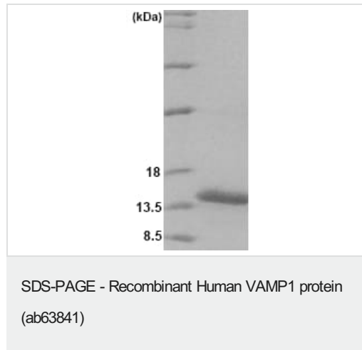
15% SDS PAGE
