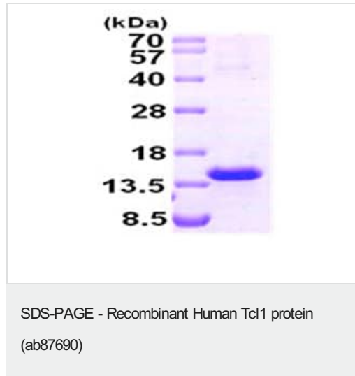
ab87690 on 15% SDS-PAGE (3µg)
