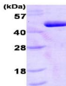
SDS-PAGE - Recombinant Human PDK1 protein (ab86986)
