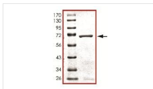
SDS-PAGE - Recombinant human p38 beta/MAPK11 protein (ab125663)
