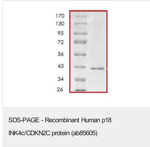
SDS-PAGE showing ab85605 at approximately 42kDa.
