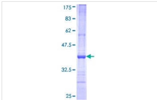
12.5% SDS-PAGE showing ab116819 at approximately 35.42kDa. Stained with Coomassie Blue.
