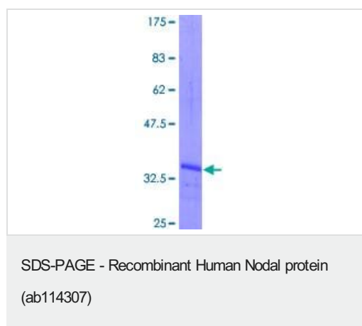
12.5% SDS-PAGE image showing ab114307 Stained with Coomassie Blue.
