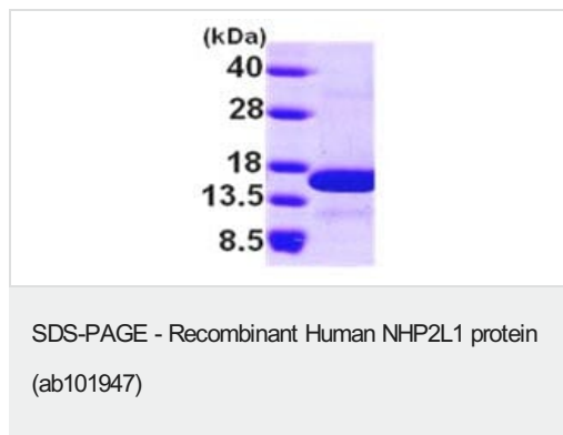
15% SDS-PAGE analysis of 3µg ab101947.
