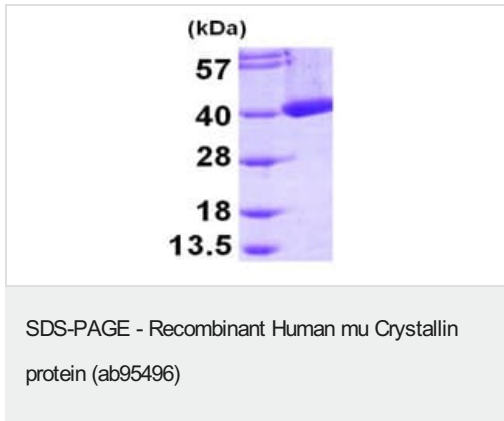
15% SDS-PAGE analysis of 3µg ab95496.
