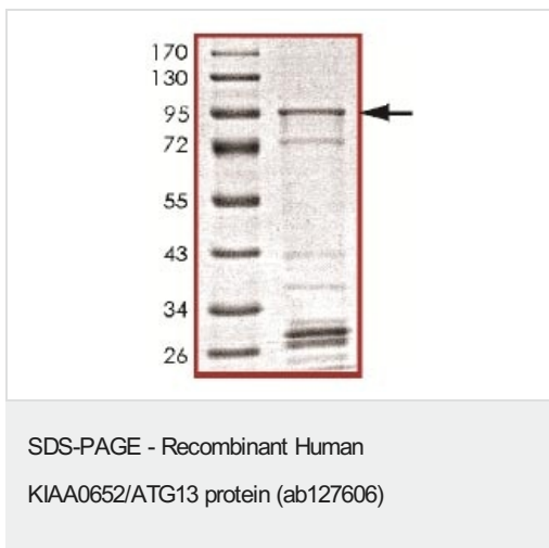
SDS-PAGE analysis of ab127606.
