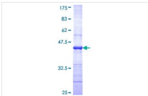
ab114174 on a 12.5% SDS-PAGE Stained with Coomassie Blue.
