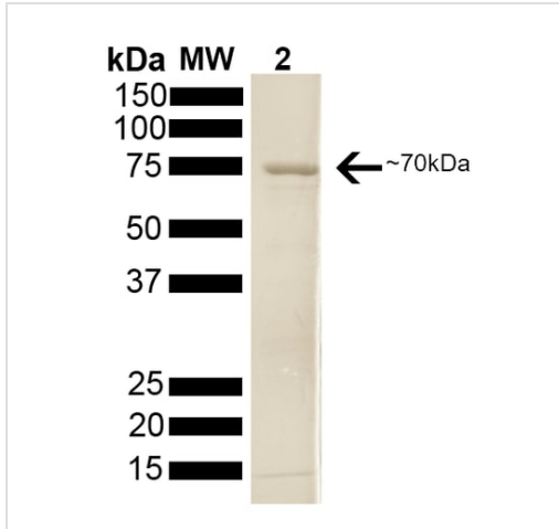
SDS-PAGE of 70kDa Hsp70 protein.
