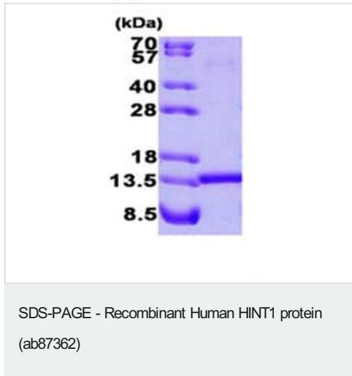
ab87362 on 15% SDS-PAGE (3 \mu g)
