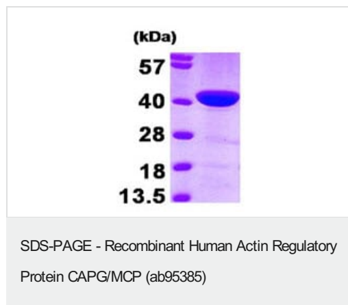
15% SDS-PAGE analysis of 3µg ab95385.
