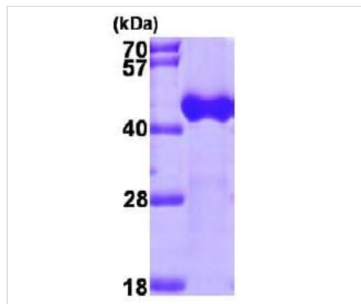
15% SDS-PAGE analysis of 3µg ab98236
