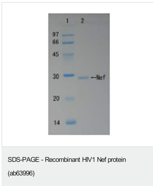
Polyacrylamide gel electrophoresis of ab63996.
