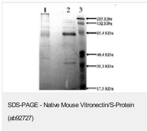
10% SDS-PAGE showing ab92727 Lane 1 ab92727 Non-reduced (3µg) Lane 2 ab92727 Reduced (3µg) Lane 3 Molecular weight markers
