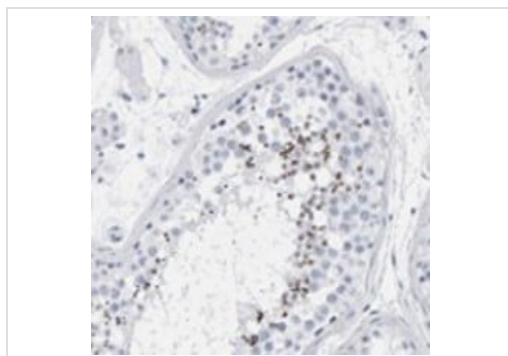
ab121768 at a 1/2500 dilution staining SPACA3 in paraffin embedded Human testis tissue by Immunohistochemistry.
