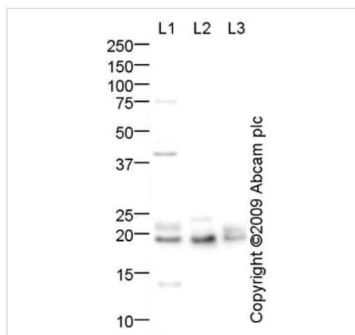
Western blot - Anti-Cytochrome b245 Light Chain/p22-phox antibody (ab75941)
