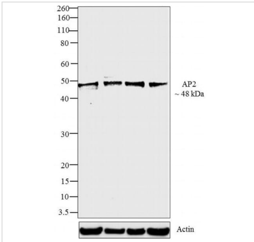
Western blot - Anti-AP2 gamma/TFAP2C antibody [3B5] (ab110635)
