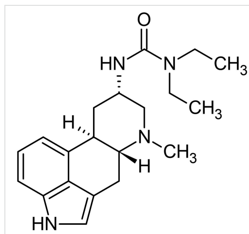
Chemical Structure - Terguride, Partial D2 agonist (ab144611)
