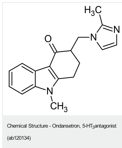
2D chemical structure image of ab120134, Ondansetron, 5-HT 3 antagonist
