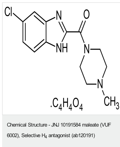
2D chemical structure image of ab120191, JNJ 10191584 maleate (VUF 6002), Selective H 4 antagonist
