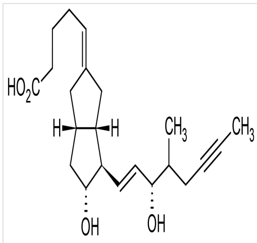
Chemical Structure - Iloprost, Prostaglandin (PGI 2 ) analog (ab120911)
