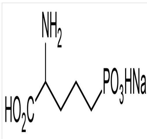
Chemical Structure - DL-AP5 sodium salt, NMDA glutamate site antagonist (ab120271)
