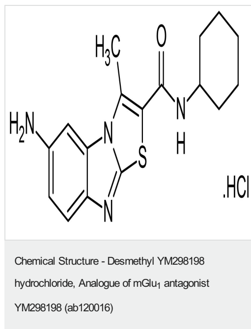
2D chemical structure image of ab120016, Desmethyl YM298198 hydrochloride, Analogue of mGlu 1 antagonist YM298198
