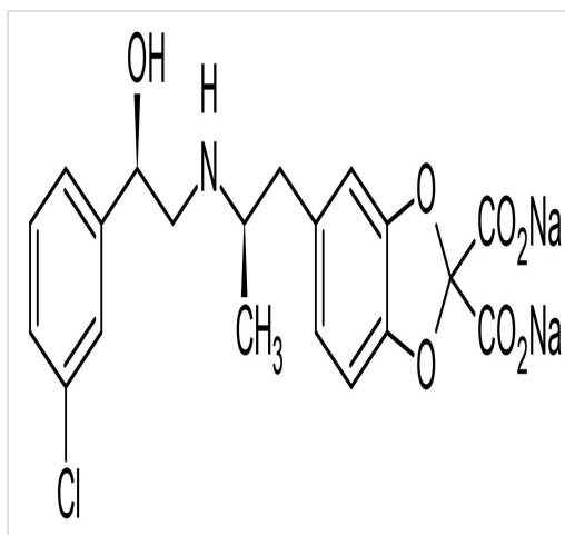
Chemical Structure - CL-316243 disodium salt, adrenergic-beta 3 receptor agonist (ab144605)
