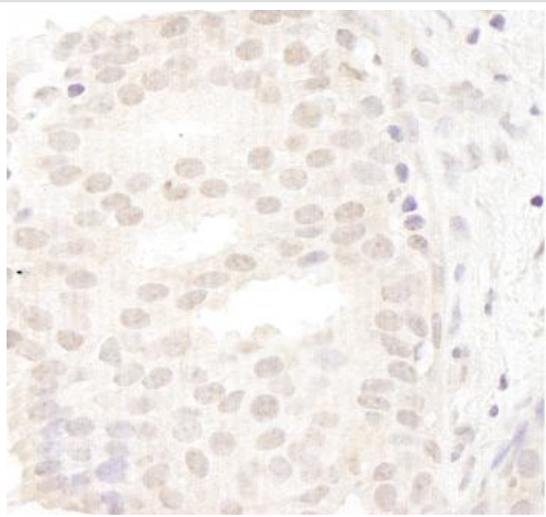
Immunohistochemistry (Formalin/PFA-fixed paraffin-embedded sections) - CASC5 antibody (ab95127)
