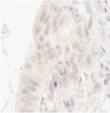
Immunohistochemistry (Formalin/PFA-fixed paraffin-embedded sections) - CASC5 antibody (ab95127)
