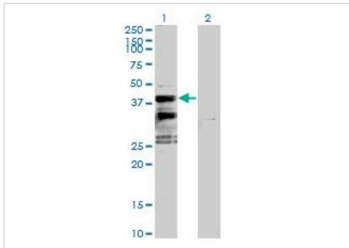
Western blot - SFXN2 antibody (ab88916)
