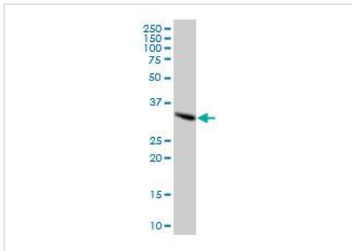
Western blot - SFXN2 antibody (ab88916)
