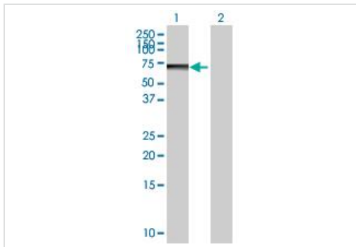
Western blot - PHF23 antibody (ab67947)
