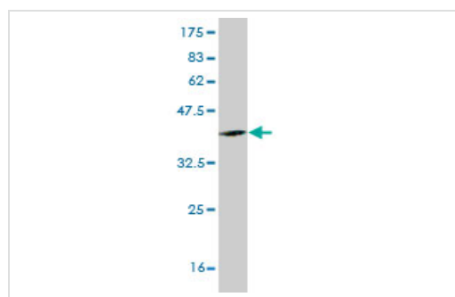
Western blot - RBMS2 antibody (ab58342)
