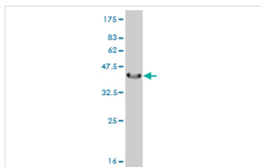
Western blot - Guanylyl Cyclase alpha 1 antibody (ab55215)
