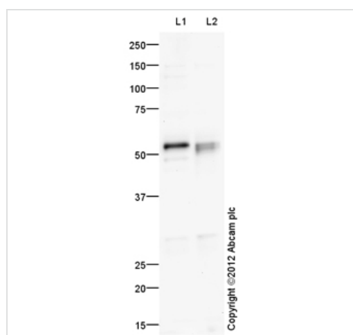
Western blot - Anti-SOX8 antibody (ab104245)
