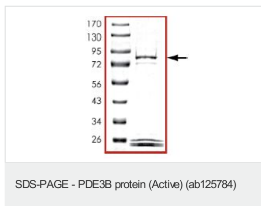
SDS-PAGE analysis of ab125784.
