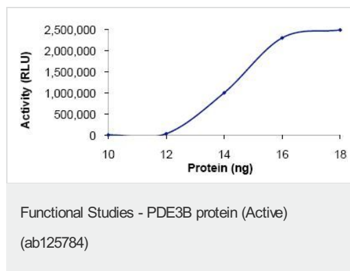
Sample assay showing the specific activity of ab125784 to be 156 nmol/min/mg.
